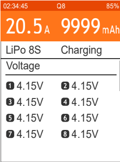
Cell voltage
